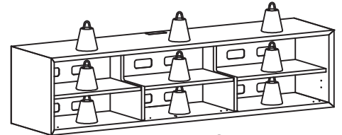
clic 230S = 70kg clic 231S = 70kg clic 232S = 70kg
